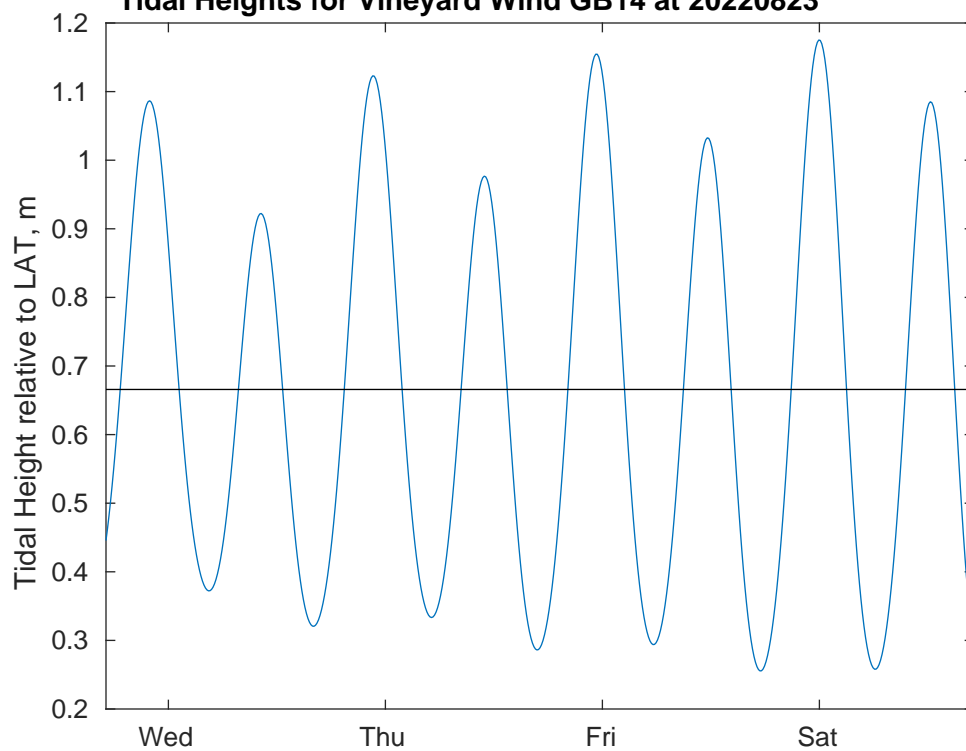
Tidal Heights for Vineyard Wind GB14 at 20220823
